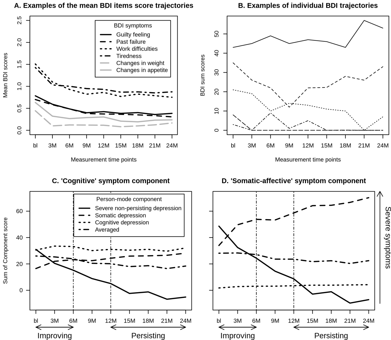
Fig 1. A. Examples of the mean BDI item score trajectories ('general trend'), B. Examples of five patients' individual BDI trajectories, C. Cognitive symptom-component plot around the general trend and D. Somatic-ffective symptom-component plot around the general trend for the three person-mode components. The two vertical lines in panels 3 and 4 indicate the divisions between the two time-components (improving and persisting).
